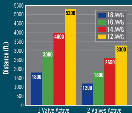
Maximum Distance From Controller Per Wire Gauge
